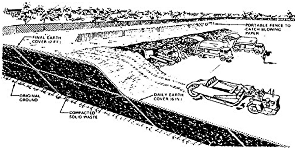
Figure 1 Typical Area Landfill Operation
