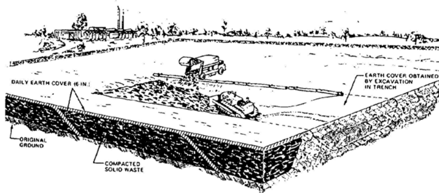
Figure 2 Typical Trench Landfill Operation
