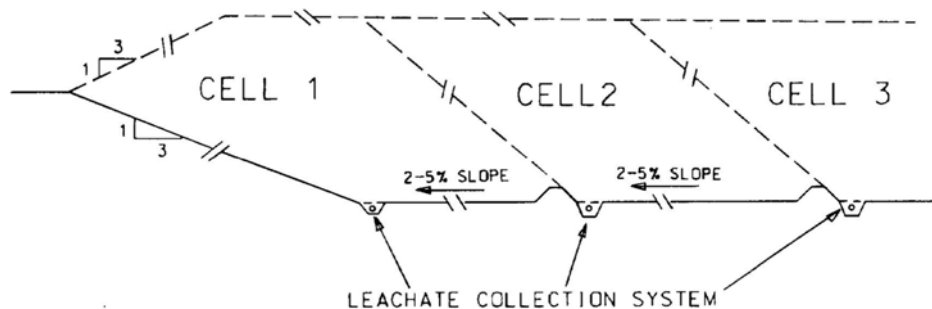
Figure 4 Typical Trench Bottom Separated by Berms
